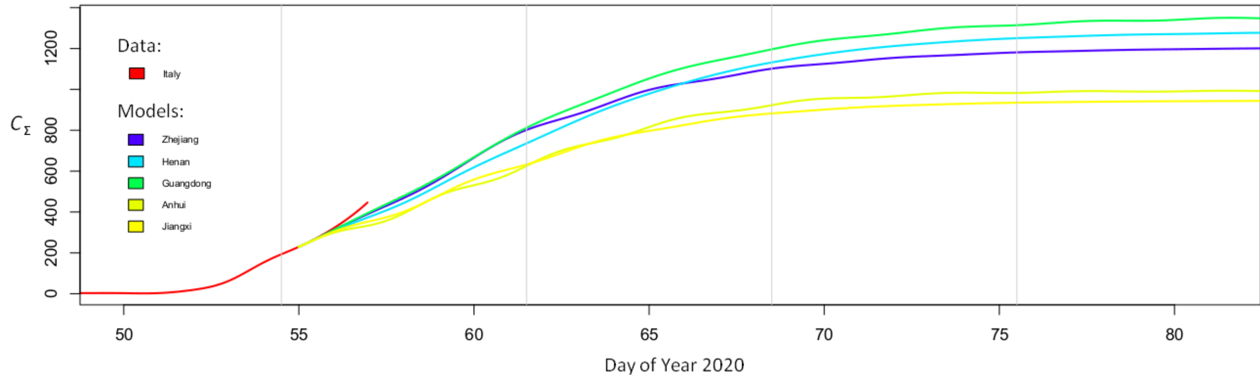
Observed and Forecasts of the Culmulated Cases of Covid-19 infection in Italy
